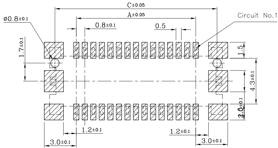
PCB PATTREN LAYOUT
